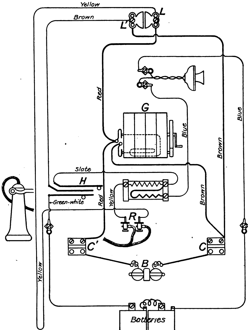
FIG. 81.—Circuit, local battery telephone, Sumter type.
